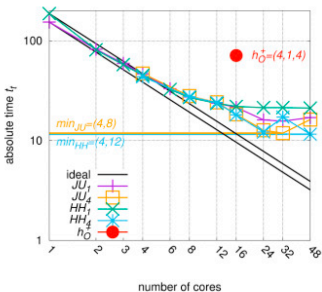
(a) Strong scaling of 100 iteration of the LBM on a single JURECA (JU) and HAZEL HEN (HH) node using the mesh with c_2 = 8.89 \cdot 10^6 cells. Furthermore, the single result at h_O^+ = (4, 1, 4) for the ODROID-MC1 is displayed. For the HPC systems the run times are shown for a single MPI rank and for four MPI ranks (indices 1 and 4).
